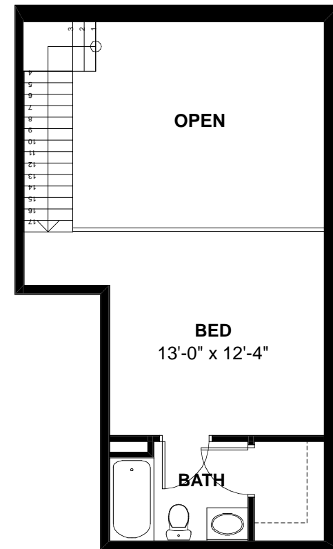
2nd floor
