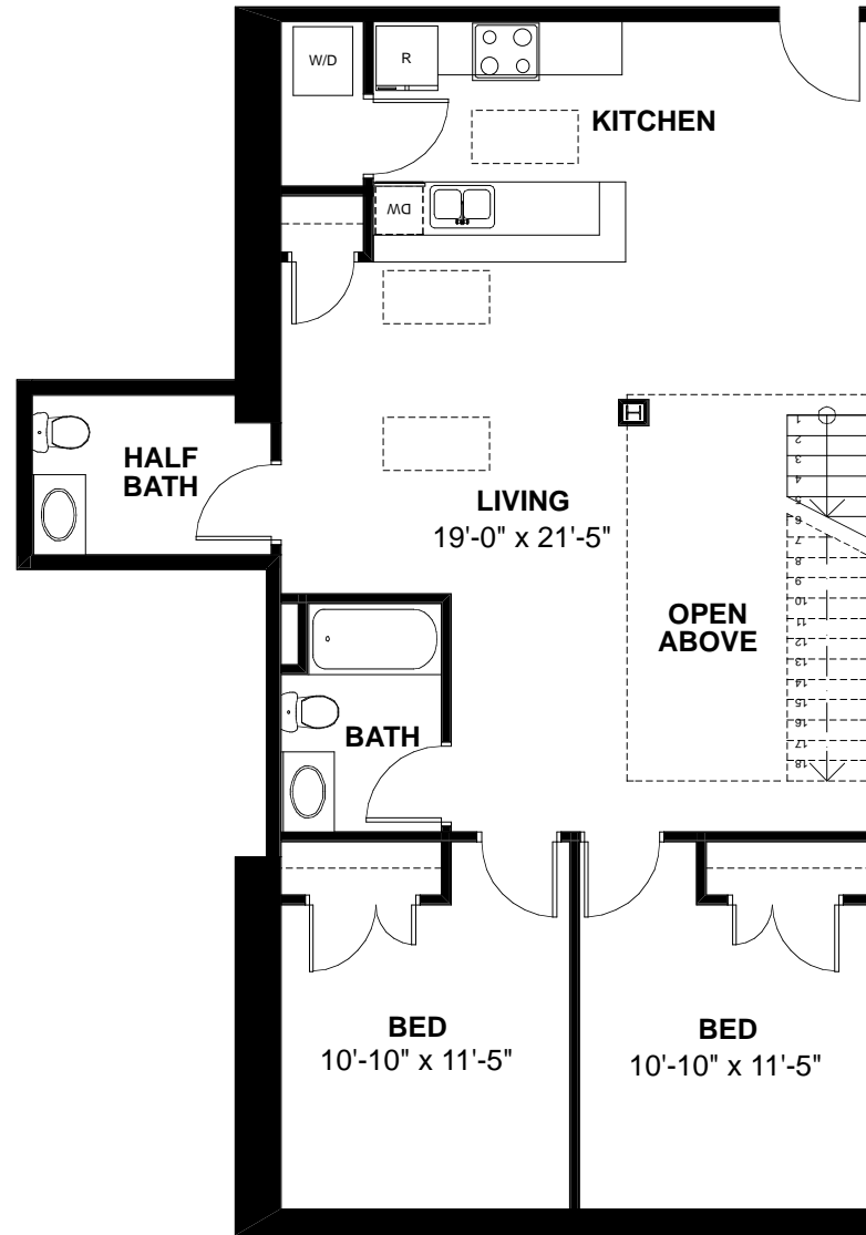
1st floor
